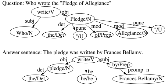
Figure 2. The dependency trees produced by MINIPAR for a question and a candidate answer sentence.
