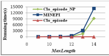
Fig. 8. Running time vs L
