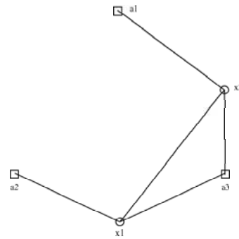
Figure 3: A strongly localizable network
