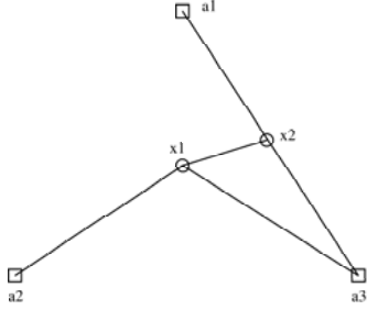
Figure 1: A uniquely localizable, but not strongly localizable network G_1
