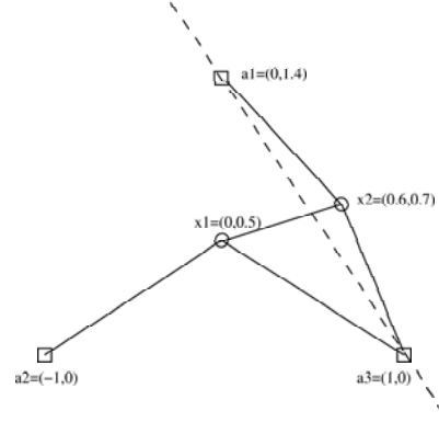
Figure 2: A rigid network that is not uniquely localizable
